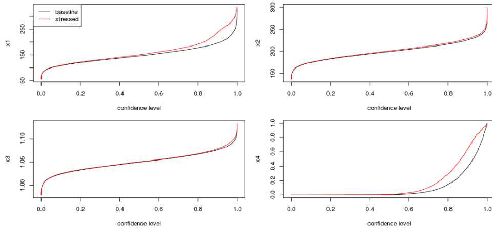
Figure 1.4: Visualisation of reverse sensitivity testing for an illustrative example
